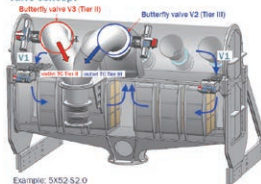
Catalytic Element
